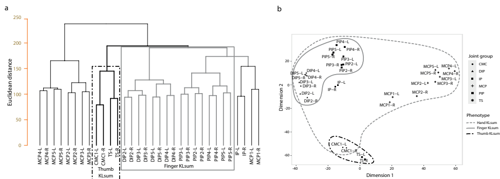
▲ Figure 1: Tree-dendrogram and multidimensional scaling (MDS) plot of KL scores in the joints of the hand. a. tree-dendrogram of complete hierarchical clustering of Euclidean distance matrix of KL scores of groups of joints. Joints were grouped per ‘type’ and per hand, left or right. b. MDS plot of KL scores for all hand joints left (L) and right (R), not grouped per “type”. Data consisted of all available data from RSI, RSII and RSIII (n=8,691). Selected clusters are depicted by the different dashed lines. OA: osteoarthritis, KL: Kellgren-Lawrence OA severity score, TS: trapezioscapoid joints, CMC: carpometacarpal joints, PIP: proximal interphalangeal joints, DIP: distal interphalangeal joints, MCP: metacarpophalangeal joints and IP: interphalangeal joints. L/R: left or right joint, number denotes which joint, i.e., PIP2L: the second PIP joint at the left hand. See supplementary figures 2-3 for dendrogram and MDS plots for joint space narrowing and osteophytosis.
