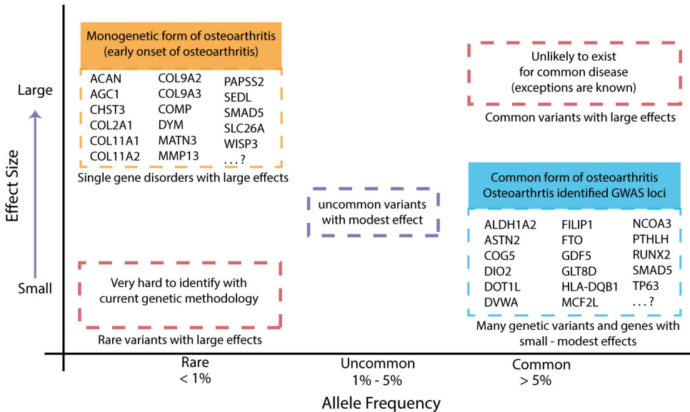
▲ Figure 4: Allele frequency and osteoarthritis disease risk. Early onset osteoarthritis or Mendelian/monogenic forms of osteoarthritis, are caused by single gene mutations. Such genetic variants have large effects, but are rare in the population. Known genes with rare mutations that give rise to early onset osteoarthritis are given in the box. For late onset or the common form of osteoarthritis, many variants and genes confer risk. Meaning that almost all of these variants must have small to moderate effect sizes. Thus common variants with large effect sizes are unlikely to exist for common diseases, although it is possible. In the box known GWAS identified loci associated with osteoarthritis are given. Figure adapted from [34, 42]
