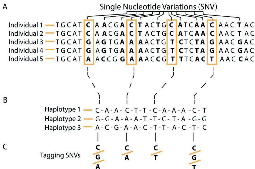
▲ Figure 5: Single Nucleotide Variants, Haplotypes, Imputation and Tagging SNVs. A) 5 short stands of DNA from four versions of the same genetic location in 5 different individuals. Most of the DNA sequence is identical, except for 12 single Nucleotide Variations (SNV) nucleotide variations (SNVs). Each SNV has several possible alleles (A/T/G/C). B) From the 5 individuals DNA sequence, 3 haplotypes can be distinguished. A haplotype is made up of a particular combination of alleles that are inherited together (in linkage). Only the SNVs are shown and 4 of them are marked. C) Tagging SNVs. By just genotyping these 4 tagging SNVs the genotype of the other 8 SNVs in linkage could be determined a.k.a. imputed, and identify these 3 haplotypes. Thus if an individual has the genotype G-A-T-G at these 4 SNVs, their haplotype would be determined as number 2. Note that haplotypes can occur at different frequencies in different populations, haplotype 3 in this example occurs at a lower frequency than haplotype 1 and 2. More reference sequences are needed to be able to detect other possible haplotypes, thereby determining the best tagging SNVs and thus to improve the accuracy and quality of imputation.
