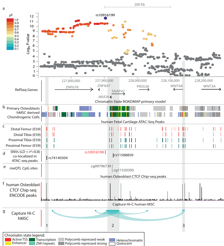
▲ Figure 3: Schematic overview of part of the rs10916199 locus. a. LocusZoom plot of rs10916199 locus, the Y-axis depicts the -\log_{10} p -value of the SNV from the thumb KLSum GWAS. Colours depict the LD ( r^2 ) between the variant and the LD SNV rs10916199. The X-axis depicts the relative genomic location, depict are the protein coding genes at those genomic locations. For this genomic region depicted in figure b – g are several epigenetic annotations are plotted. b. Chromatin state, as predicted by the ROADMAP 15-state model on histone modifications, for primary osteoblasts and human mesenchymal stem cell derived chondrocytes. Colours depict chromatin states, legend at bottom of full figure. c. ATAC-seq peaks from human embryonic cartilage at different bone development sites at gestation day (E)59. d. Location of the lead SNV, rs10916199 and two putative causal SNV's which co-locate with ATAC-seq peaks. e. Genomic location of rs10916199 meQTL CpG sites. f. Chip-seq CTCF protein binding peaks from human primary osteoblasts from ENCODE. g. Capture Hi-C chromatin interactions from 3D genome browser for human mesenchymal Stem Cells (hMSC) and mesoderm. Depicted are the chromatin interactions from the promoters of the queried gene to the genomic location of interaction, this was done for the JMJD4/SNAP47 transcription start site (TSS), WNT9A TSS and the WNT3A TSS. For details on methods and underlying data see supplementary methods.
